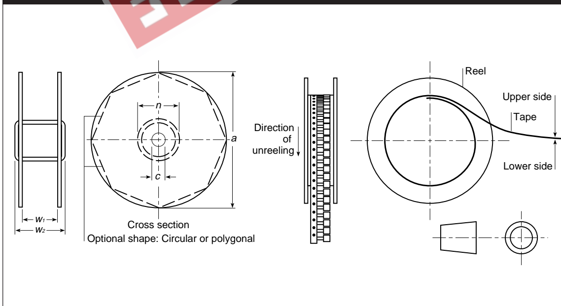
Figure 2: Reel Dimensions
