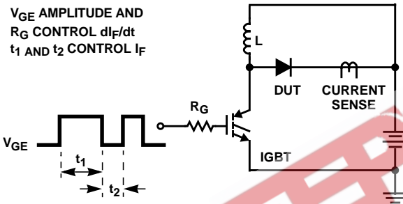
FIGURE 5. t_{rr} TEST CIRCUIT
