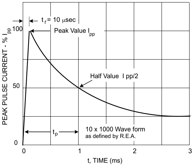
Fig. 1, Pulse Waveform
