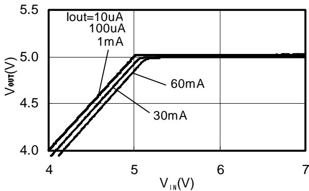
S-818A50A (Ta=25°C)
