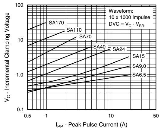
Figure 10. Incremental Clamping Voltage Curve Bi-Directional
