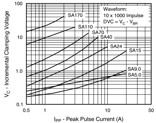
Figure 8. Incremental Clamping Voltage Curve Uni-Directional
