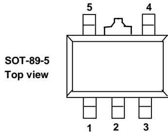
Figure 3 SOT-89-5
