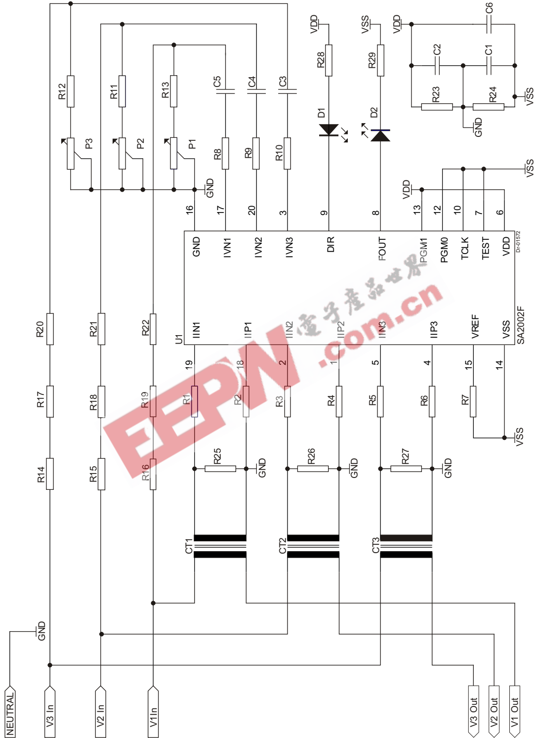
Figure 5: Application Circuit
