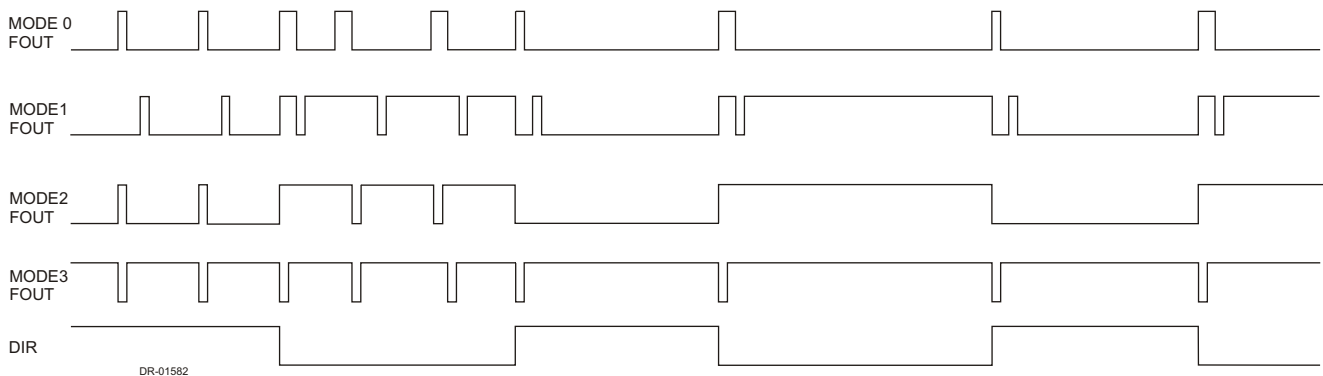
Figure 4: FOUT options
