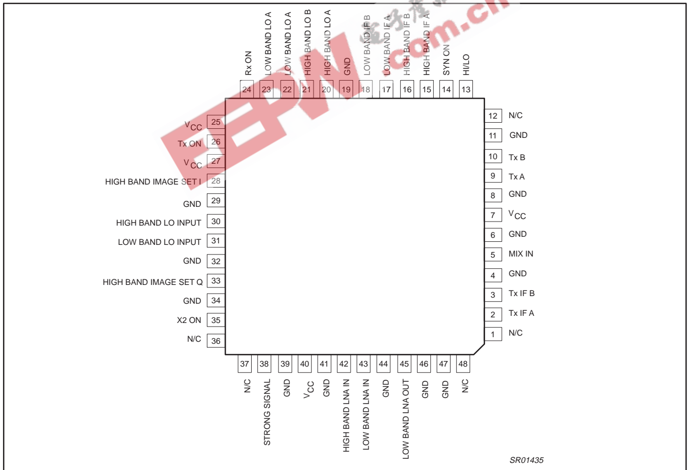
Figure 1. Pin Configuration
