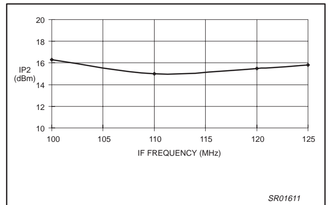
Figure 10. High Band IP2 vs. IF Frequency
