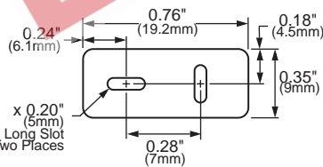
Option with Slit: Modify Beam Size of Through-Beam Sensor
