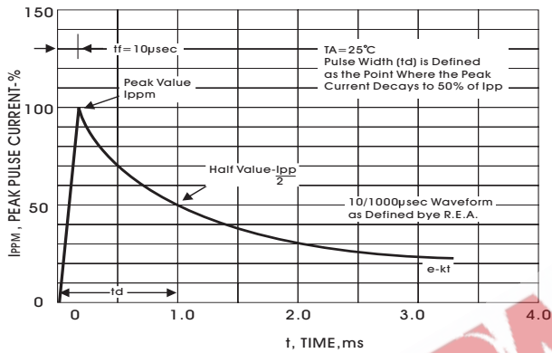
FIGURE 3-PULSE WAVEFORM
