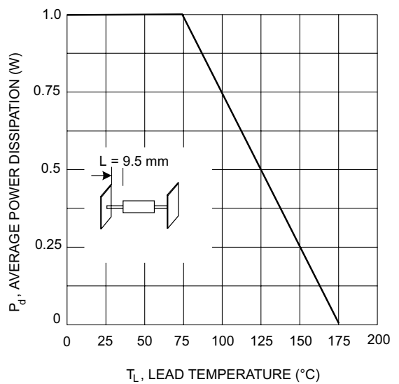
Fig. 5, Power Derating
