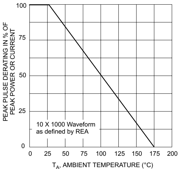
Fig. 4, Derating Curve
