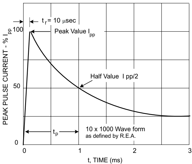
Fig. 1, Pulse Waveform
