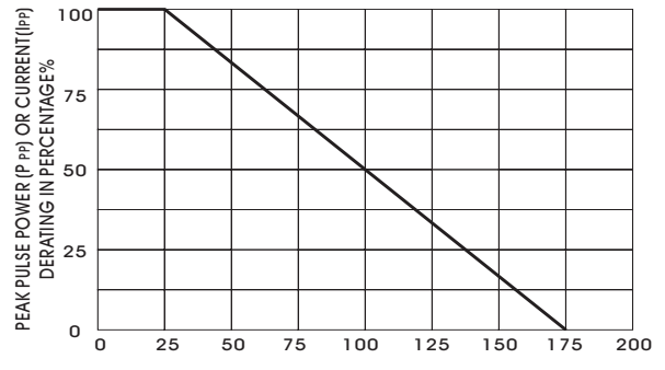
FIGURE 2-PULSE DERATING CURVE
