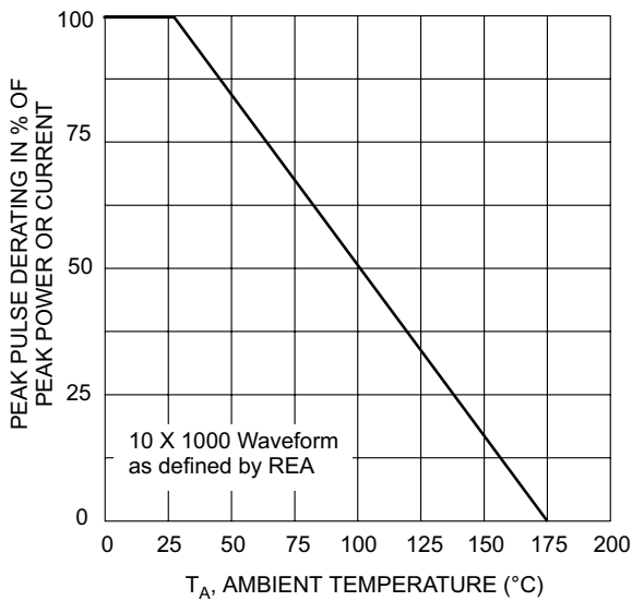
Fig. 4, Derating Curve
