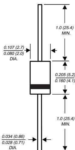
DO-204AL
