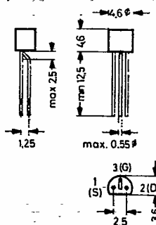
TO-92 Plastic Package Pins TO-18 "A" Weight approx. 0.18 g
