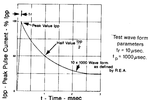
FIGURE 2 PULSE WAVEFORM
