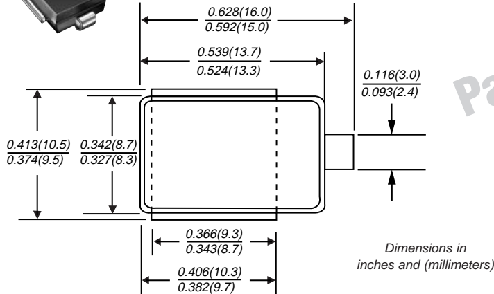
DO-218AB
