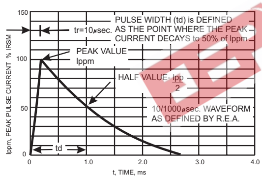
FIG.3- PULSE WAVEFORM
