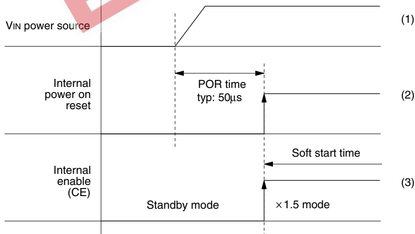
Internal reset operation when power is applied (power-ON reset)
