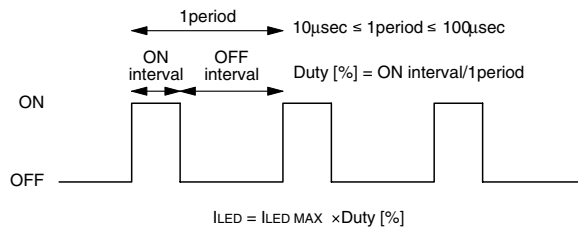
PWM duty
