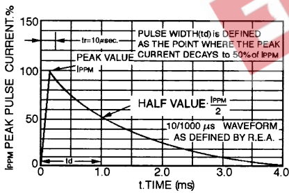
FIG. 3 - PULSE WAVEFORM
