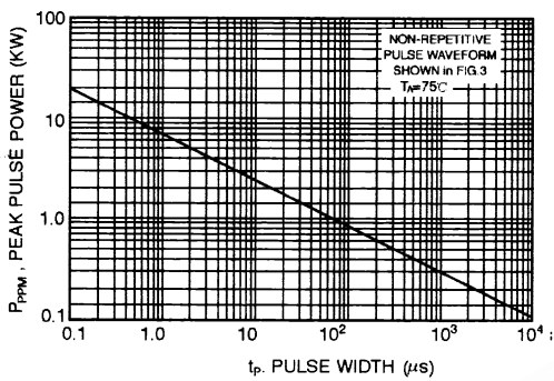
FIG. 1 - PULSE RATING CURVE
