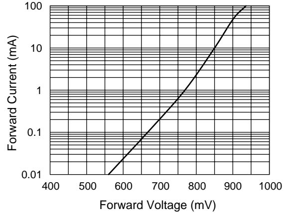
DC Characteristic
