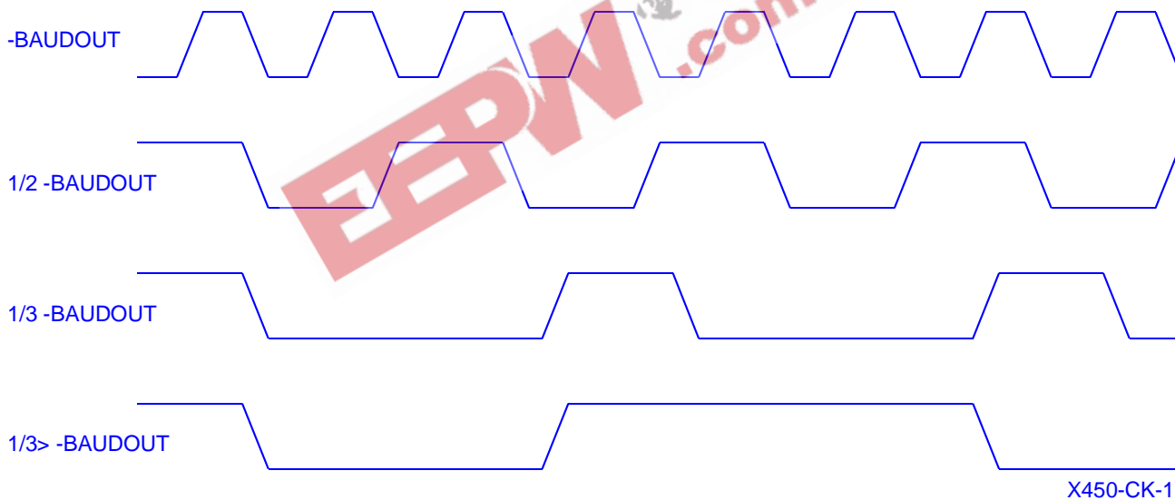
Clock timing
