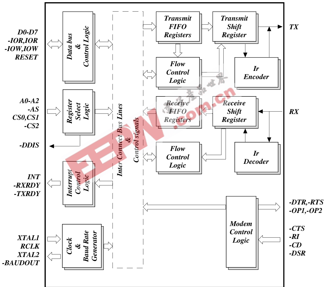
Figure 2, BLOCK DIAGRAM
