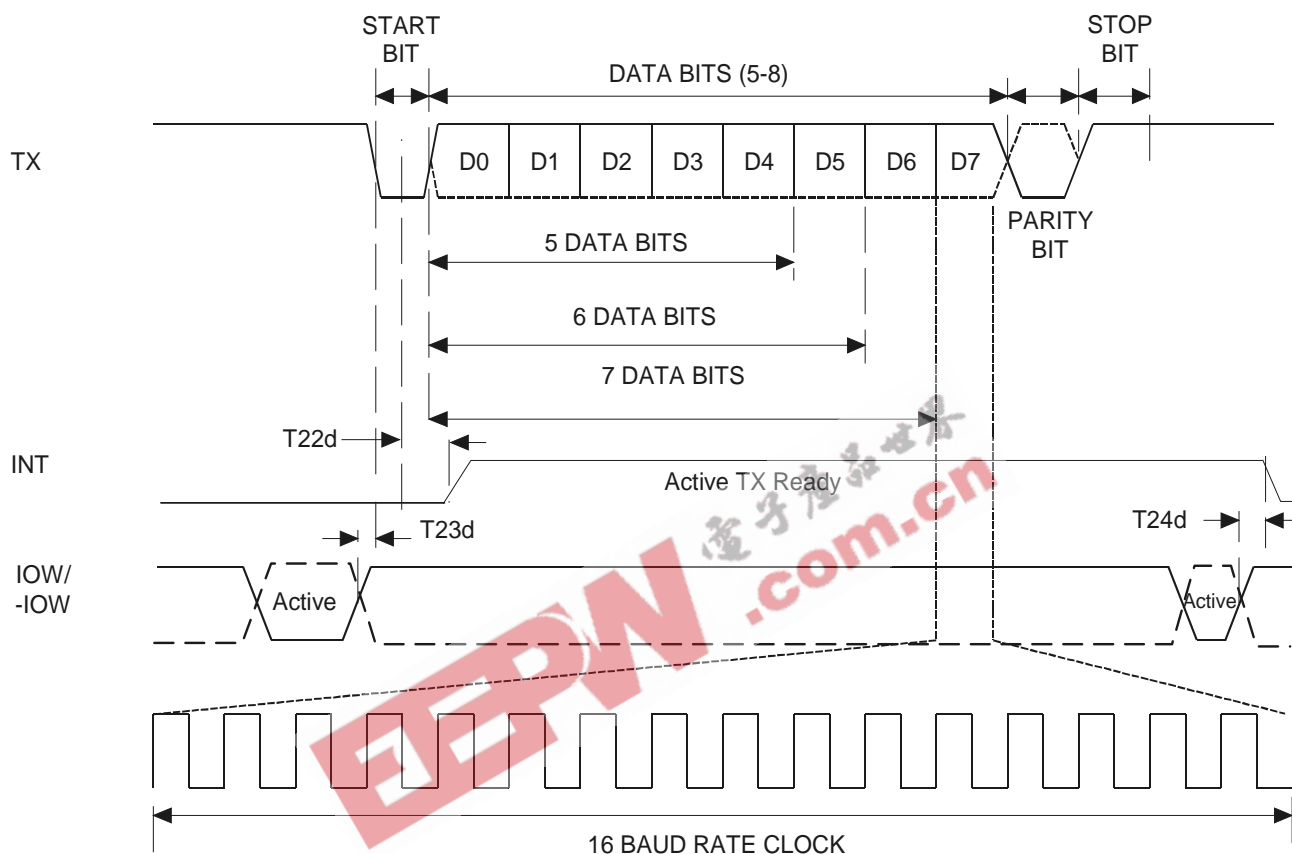
Transmit timing
