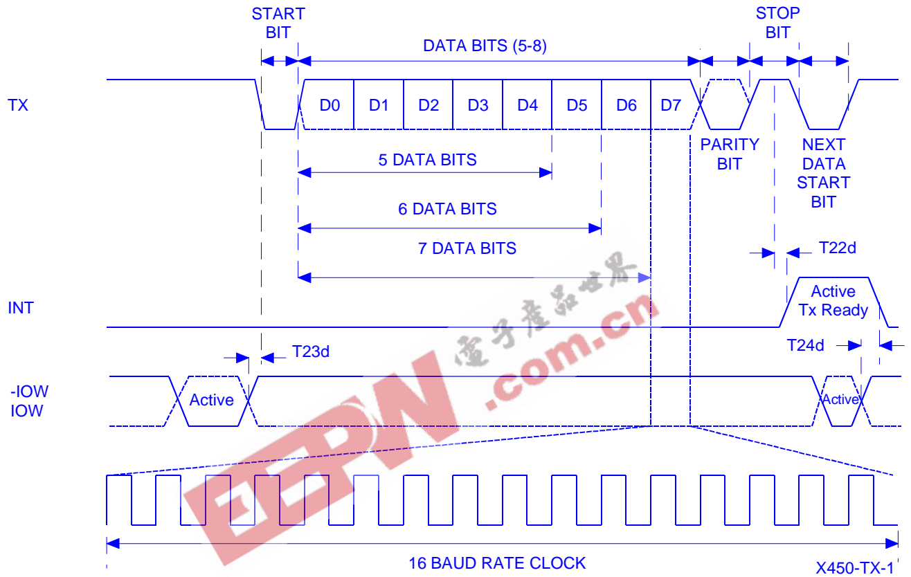
Transmit timing
