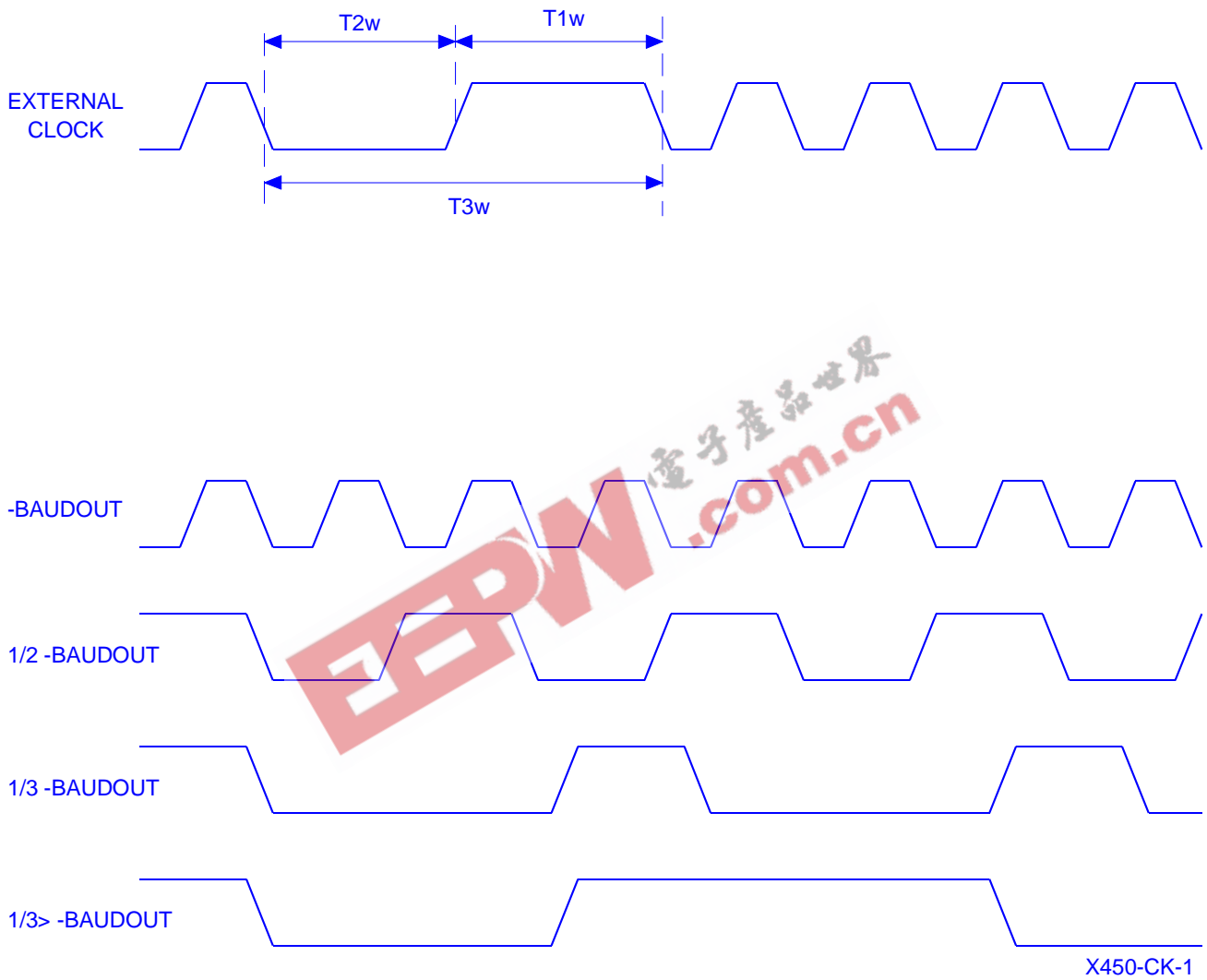
Clock timing
