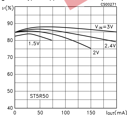
Figure 4: Typical Application Efficiency
