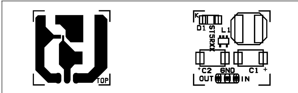
Figure 5: Typical Demoboard
