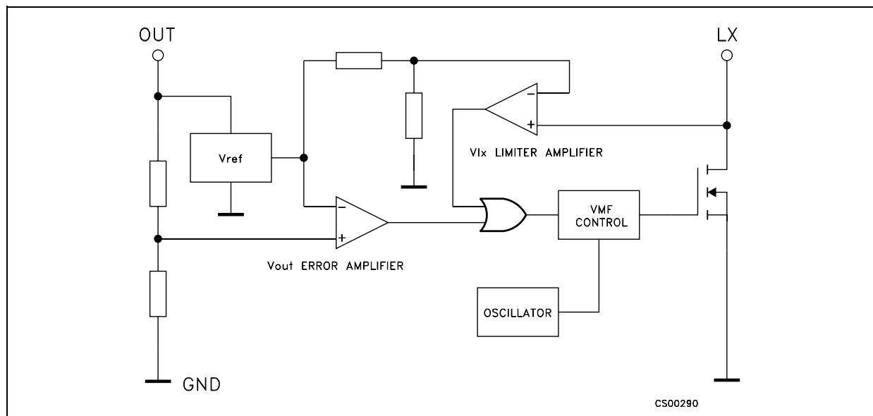
Figure 1: Schematic Diagram
