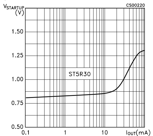
Figure 23: Start-up Voltage (V IN - V F ) vs Output Current
