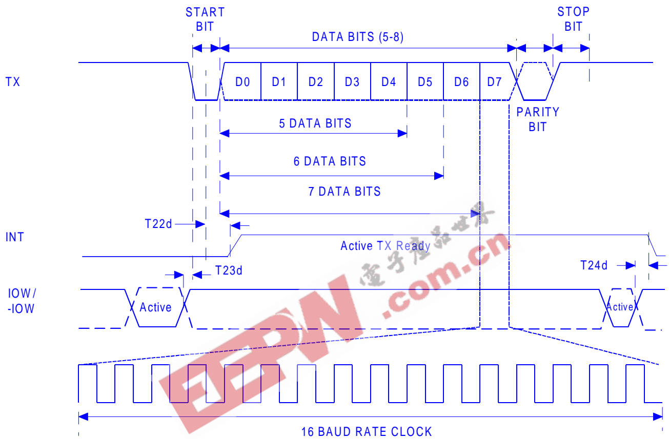
Transmit timing
