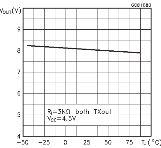
High Level Output Voltage Swing vs Temperature
