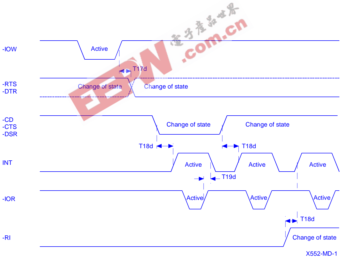
Modem input/output timing
