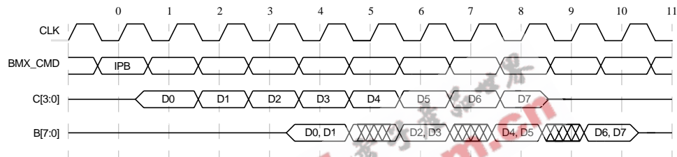
Figure 14. Block Transfer From I/O to Processor
