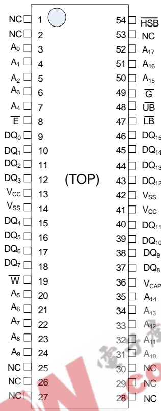
54-Pin TSOP-II
