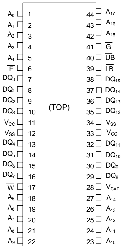
44-Pin TSOP-II
