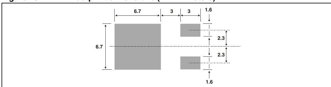
Figure 20. DPAK footprint dimensions (in millimeters)
