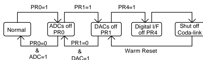
Figure 13. STAC9708/11 Powerdown/Powerup flow with analog still alive
