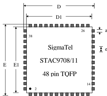
Figure 1. Package Outline
