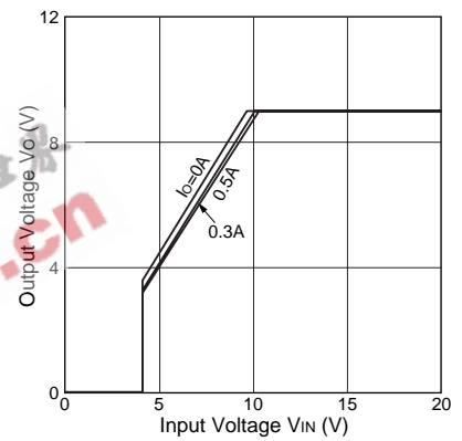
Rise Characteristics(Ch2:9V)
