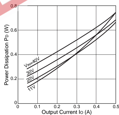
Pd Characteristics(Ch2:9V)
