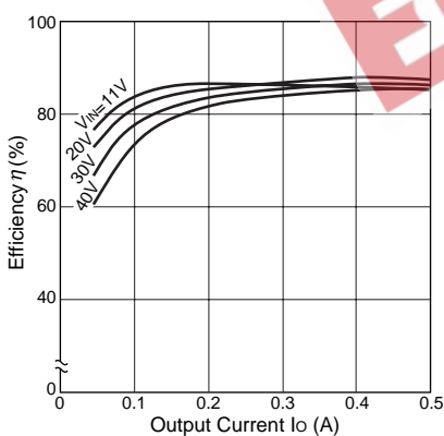
Efficiency Characteristics(Ch2:9V)
