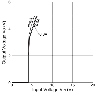
Rise Characteristics(Ch1:5V)
