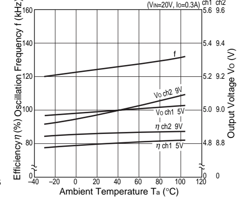
Temperature Characteristics(Ch1:5V, Ch2:9V)
