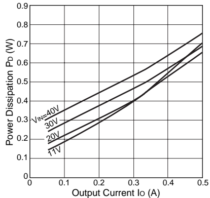
Pd Characteristics(Ch1:9V)
