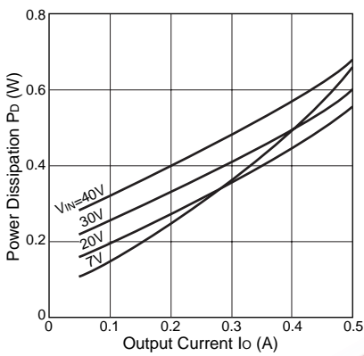
Pd Characteristics(Ch1:5V)
