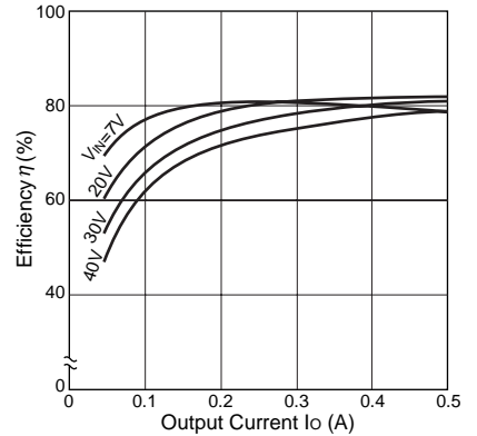
Efficiency Characteristics(Ch1:5V)
