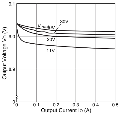
Load Regulation(Ch1:9V)
