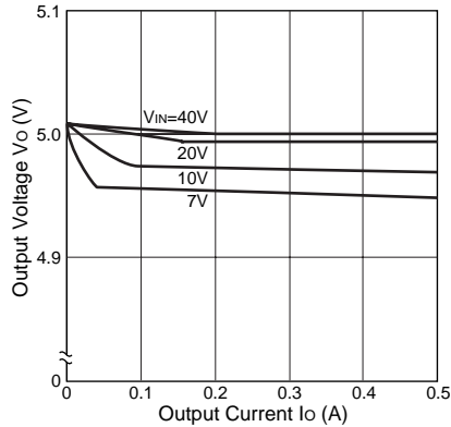
Load Regulation(Ch1:5V)
