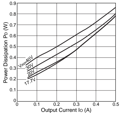
Pd Characteristics(Ch2:15.7V)
