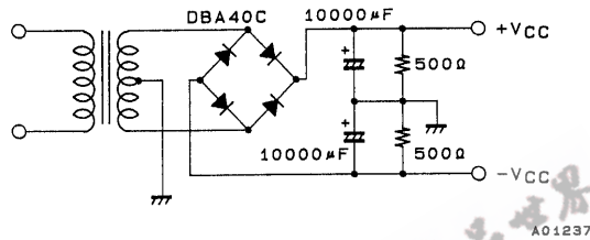
Specified Transformer Power Supply (MG-200 equivalent)
