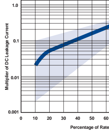
Figure 4. Typical Range of DC Leakage Current as a Function of Applied Voltage
