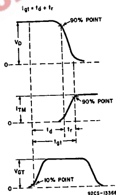
Fig. 16-Relationship between off-state voltage, on-state current, and gate-trigger voltage showing reference points for definition of turn-on time (t g ).
