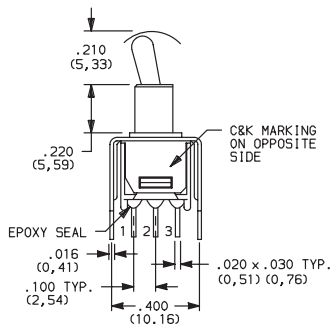
T101MH9V3BE SPDT
