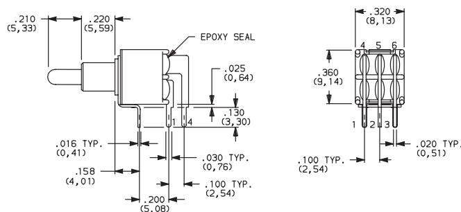
T201MH9ABE Horizontal Actuation DPDT
