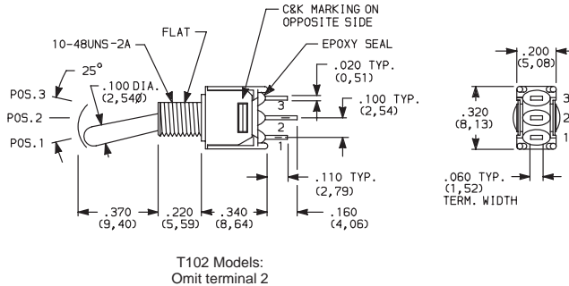
T101SHZQE SPDT
