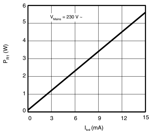
Figure 6-2. Power Dissipation of R_1 According to Current Consumption
