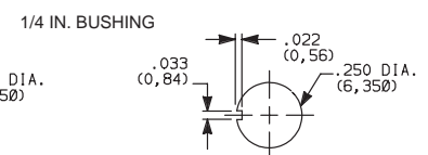
With Standard Locking Ring
