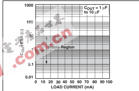
FIGURE 2-17: Stability Region vs. Load Current.
