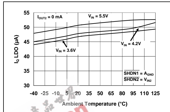
FIGURE 2-4: I_Q LDO Current vs. Ambient Temperature.
