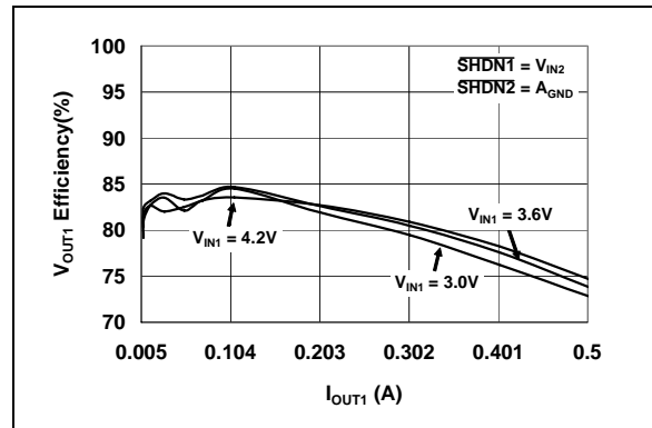
FIGURE 2-6: V_{OUT1} Output Efficiency vs. I_{OUT1} ( V_{OUT1} = 1.2V ).
