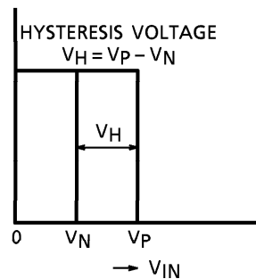
● TRANSFER CHARACTERISTICS
