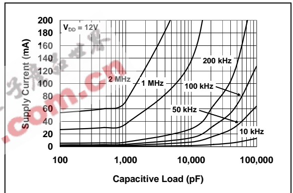
FIGURE 2-17: Supply Current vs. Capacitive Load ( V_{DD} = 12\text{V} ).
