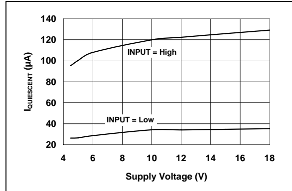
FIGURE 2-10: Quiescent Supply Current vs. Supply Voltage.
