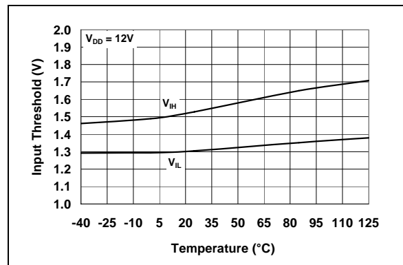
FIGURE 2-12: Input Threshold vs. Temperature.
