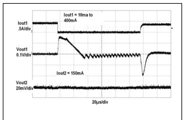
FIGURE 2-36: V_{OUT1} Load Step Response vs. Time.
