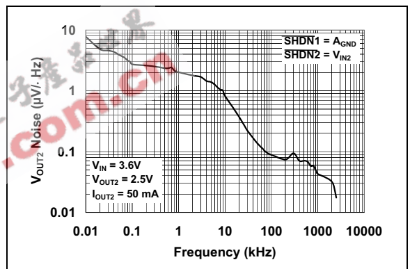
FIGURE 2-35: V_{OUT2} Noise vs. Frequency.
