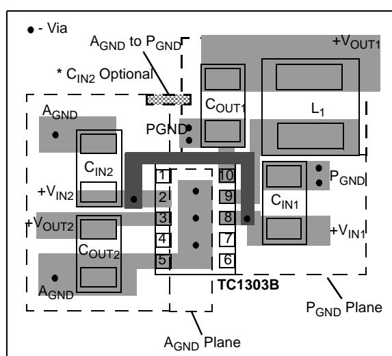
FIGURE 5-2: Component Placement, Fixed 10-Pin DFN.
