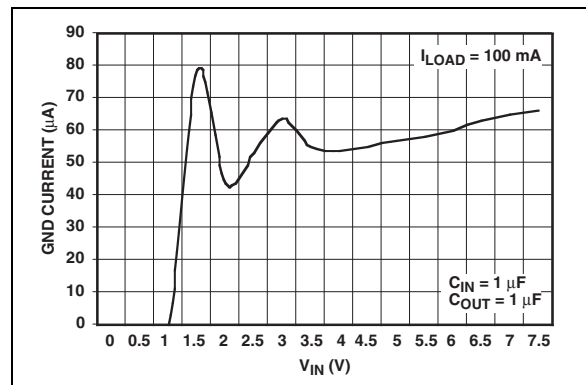
FIGURE 2-6: Ground Current vs. V_{IN} ( I_{LOAD} = 100 \text{ mA} ).
