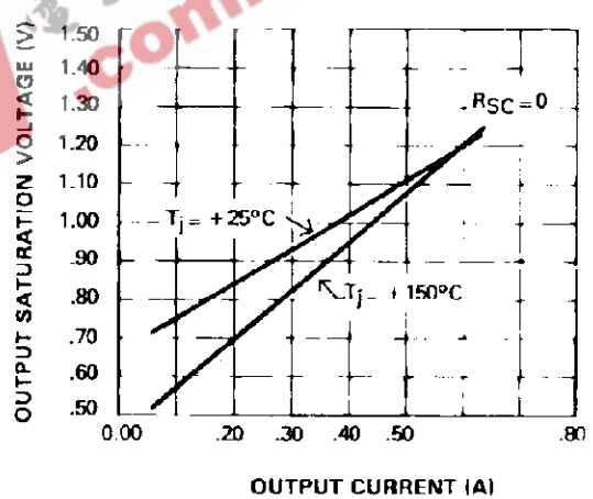
Figure 5. OUTPUT SATURATION VOLTAGE vs OUTPUT CURRENT.
