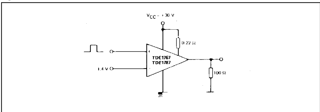
Figure 12 : Test Circuit.
