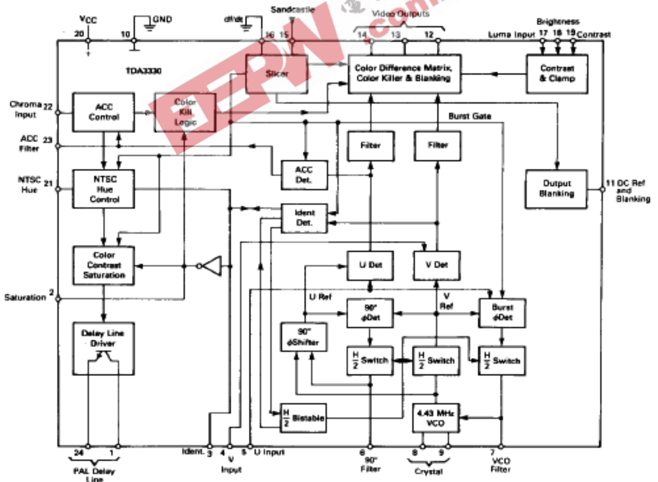
FIGURE 6 — BLOCK DIAGRAM
