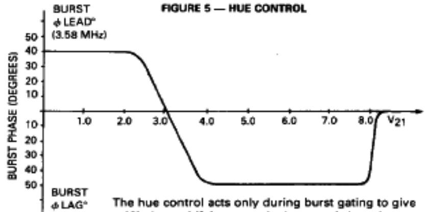
FIGURE 5 — HUE CONTROL
