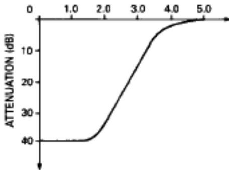
FIGURE 4 — CONTRAST CONTROL V 19 (VOLTS)
