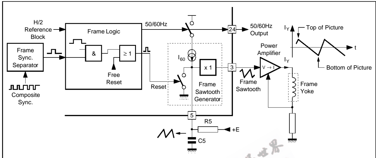
Figure 51 : Block Diagram of the Vertical Deflection Stage
