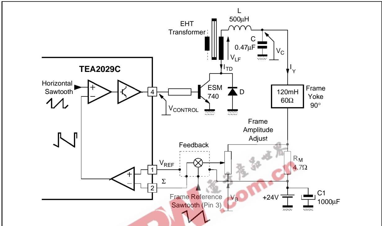
Figure 80 : Block Diagram
