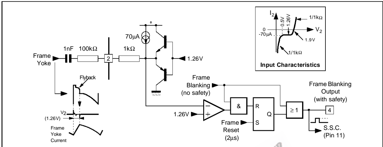
Figure 61 : Block Diagram
